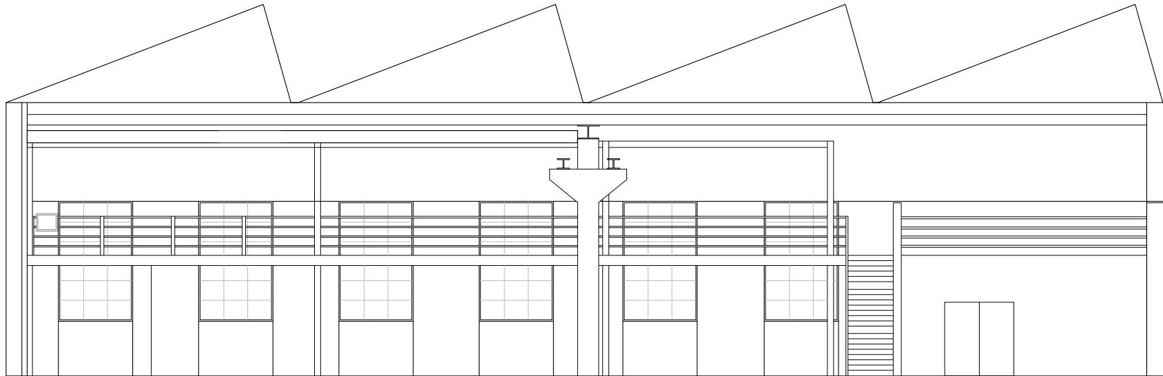
Section AA'
